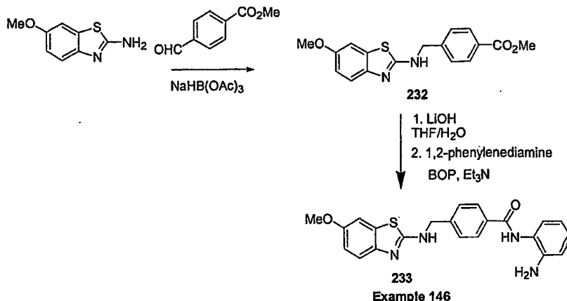
Scheme 35
